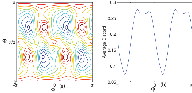
FIG. 6. (Color online) (a) Contour plot of discord for j = 40 . Blue regions indicate regions of low average discord. (b) Average discord for \theta = 2.25 and varying \phi . Comparison to classical phase space shows that chaotic region initial conditions lead to higher average discord.
