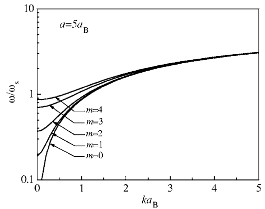
FIG. 2. The dispersion relation \omega/\omega_s of the quantum ion-acoustic wave for the nanotube's radius a=5a_B and different azimuthal quantum numbers m=0, 1, 2, 3 , and 4 .
