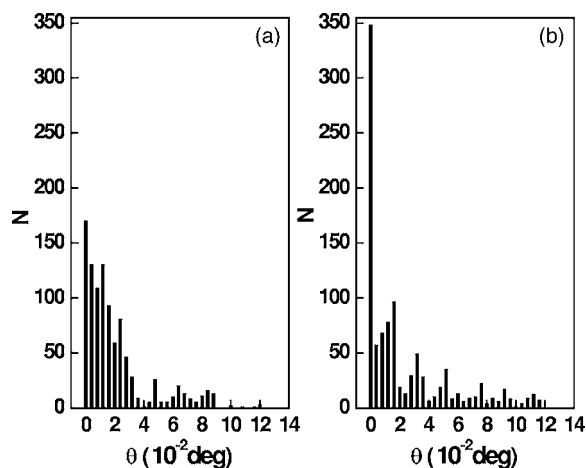
FIG. 9. The statistical distributions of the angles (a) with (b) without the dynamic polarization after the homogeneous beam traveled 10^5 a.u. through a single-wall carbon nanotube. Here the input parameters are same as those used in Fig. 8.
