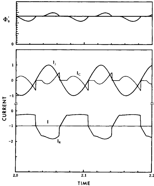
FIG. 2. (a) Portion of \Phi'(t) for T/T_c=0.7 and \beta_0=80 . At this temperature, \alpha=0.0825 , \gamma=650 , and \mathcal{R}=0.172 . Apart from a scale factor, this also is equivalent to a plot of junction voltage with the horizontal reference line corresponding to the energy gap. (b) Time dependence of the total loop current and its components flowing through the junction circuit elements.
