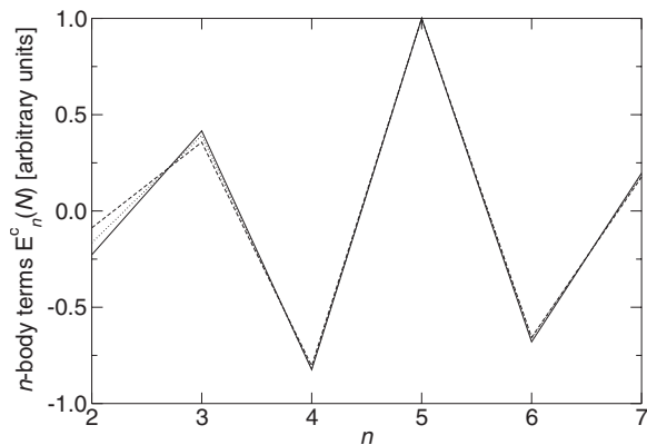
FIG. 6. Au 7 clusters: n -body expansion of the correlation energy E^c . Energy terms are normalized to the largest respective component. Solid line: D_{5h} . Dotted line: C_s . Dashed line: D_{\infty h} .
