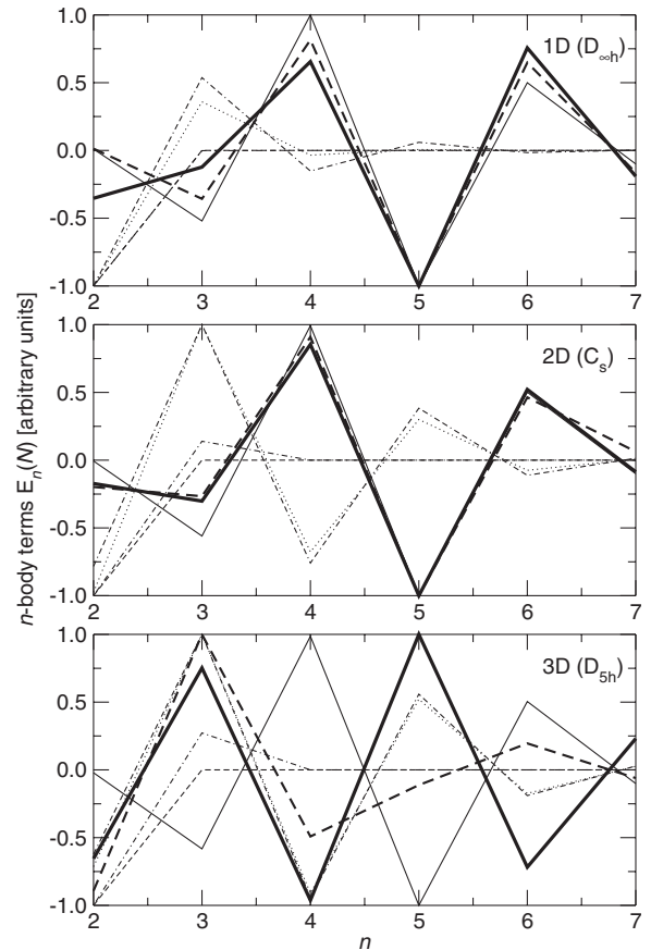
FIG. 7. Au 7 clusters: n -body expansion of interaction energies from different model potentials. From top to bottom: 1D ( D_{\infty h} ), 2D ( C_s ), 3D ( D_{5h} ). Energy terms are normalized to the largest respective component. Reference calculation: MP2 (thick solid line). Model potentials used: Lennard-Jones (dashed line), Murrell-Mottram (dash-dotted line), Gupta (dotted line), Sutton-Chen (double-dash-dotted line), Glue (solid line); PM6 method (thick dashed line).
