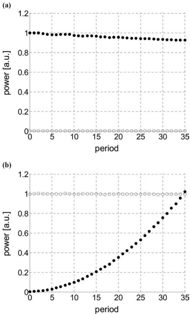
Fig. 7. Modal power evolution in the U-GACC example of Section 4. Order of grating segments: HH, HL, LL, LH . ●, mode 1; ○, mode 2. (a) Power input to mode 1: see Fig. 6, upper right figure. (b) Power input to mode 2: see Fig. 6, upper left figure.
